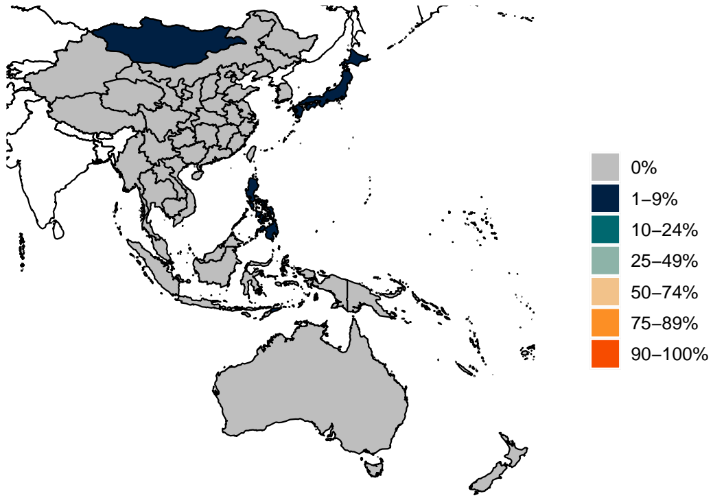
Figure 9.1: Estimated percent of new infections that are Alpha variant
