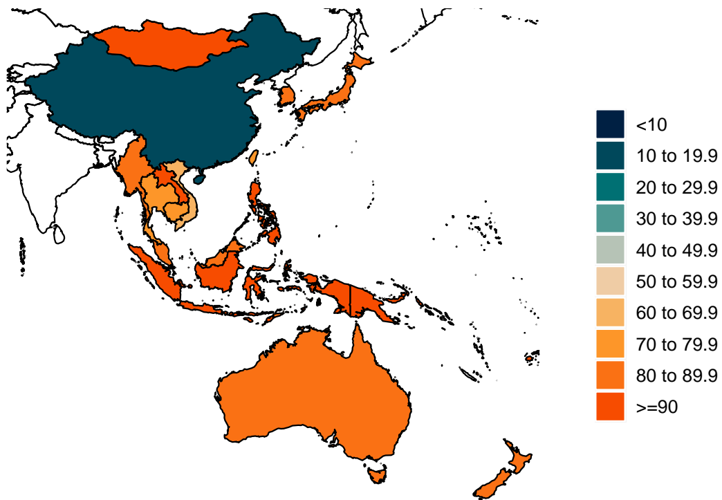
Figure 6.1: Estimated percent of the population infected with COVID-19 on December 12, 2022
